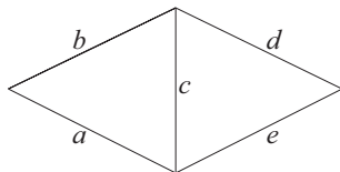
Figure 1: A graph weighted by \{a, b, c, d, e\}
