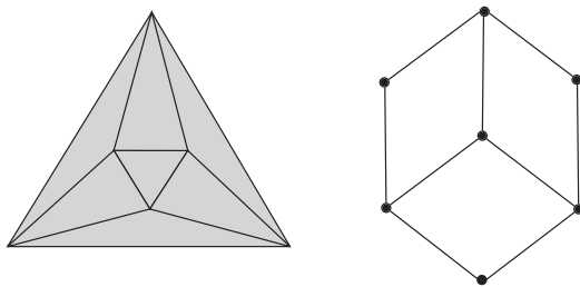
Figure 6: \Delta and its dual graph G
