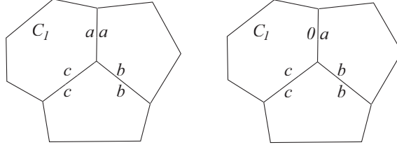
Figure 3: Removing an edge from C_1
